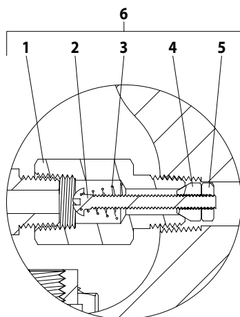
View "A"
