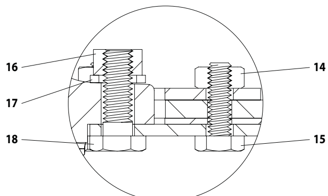
View "B"
